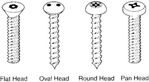
Examples of Standard- and Machine-thread Security Screws
