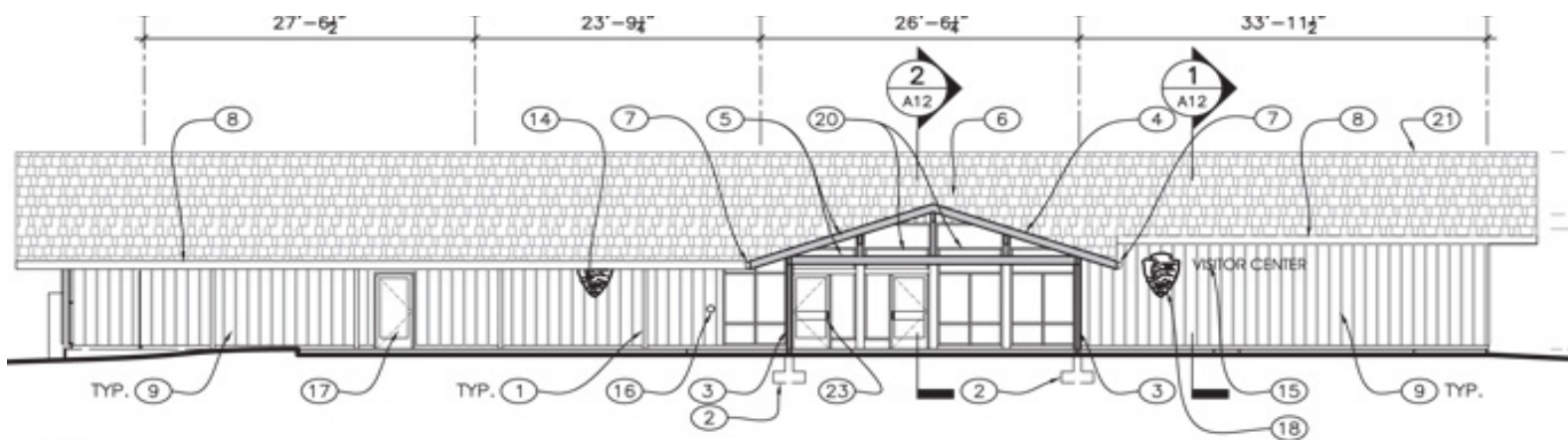
1 NORTH ELEVATION A11
